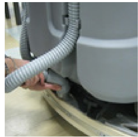
6. Install squeegee.
